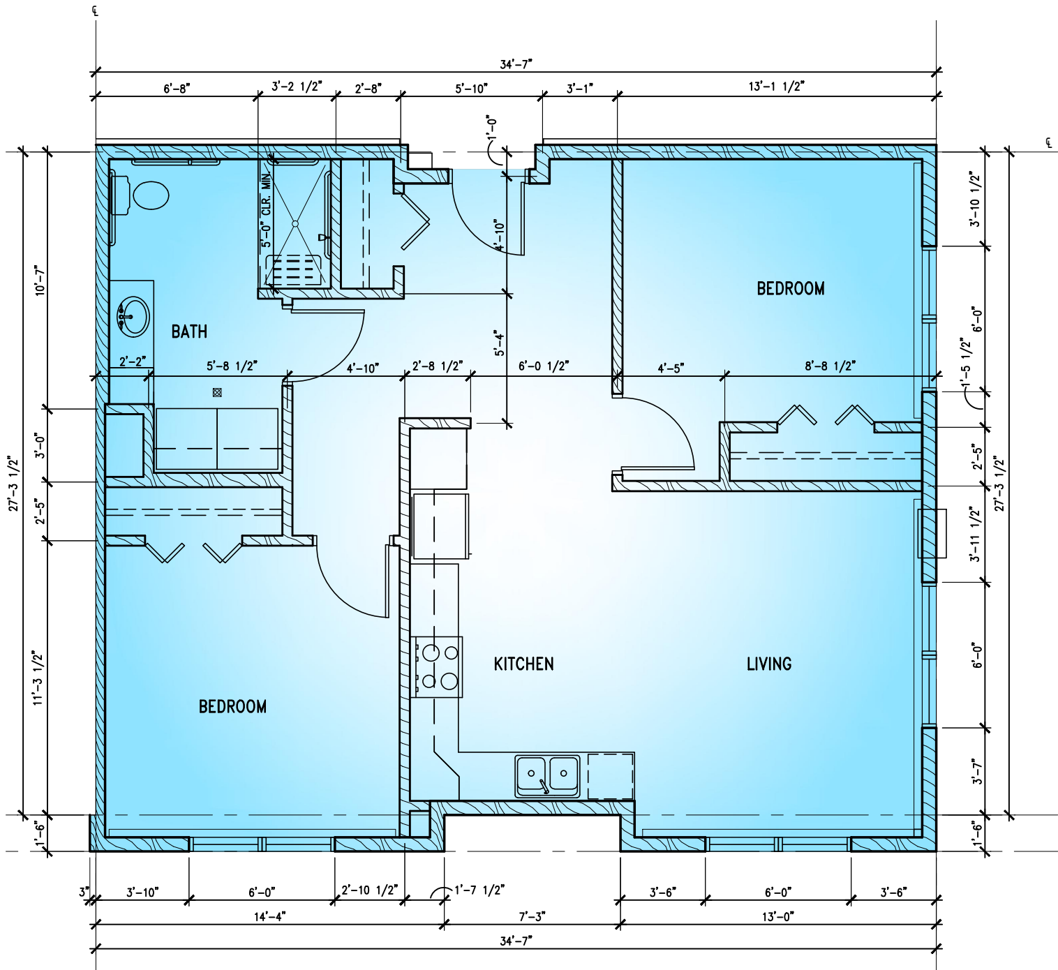
3 UNIT C-2 PLAN A340 1/4" = 1'-0"
